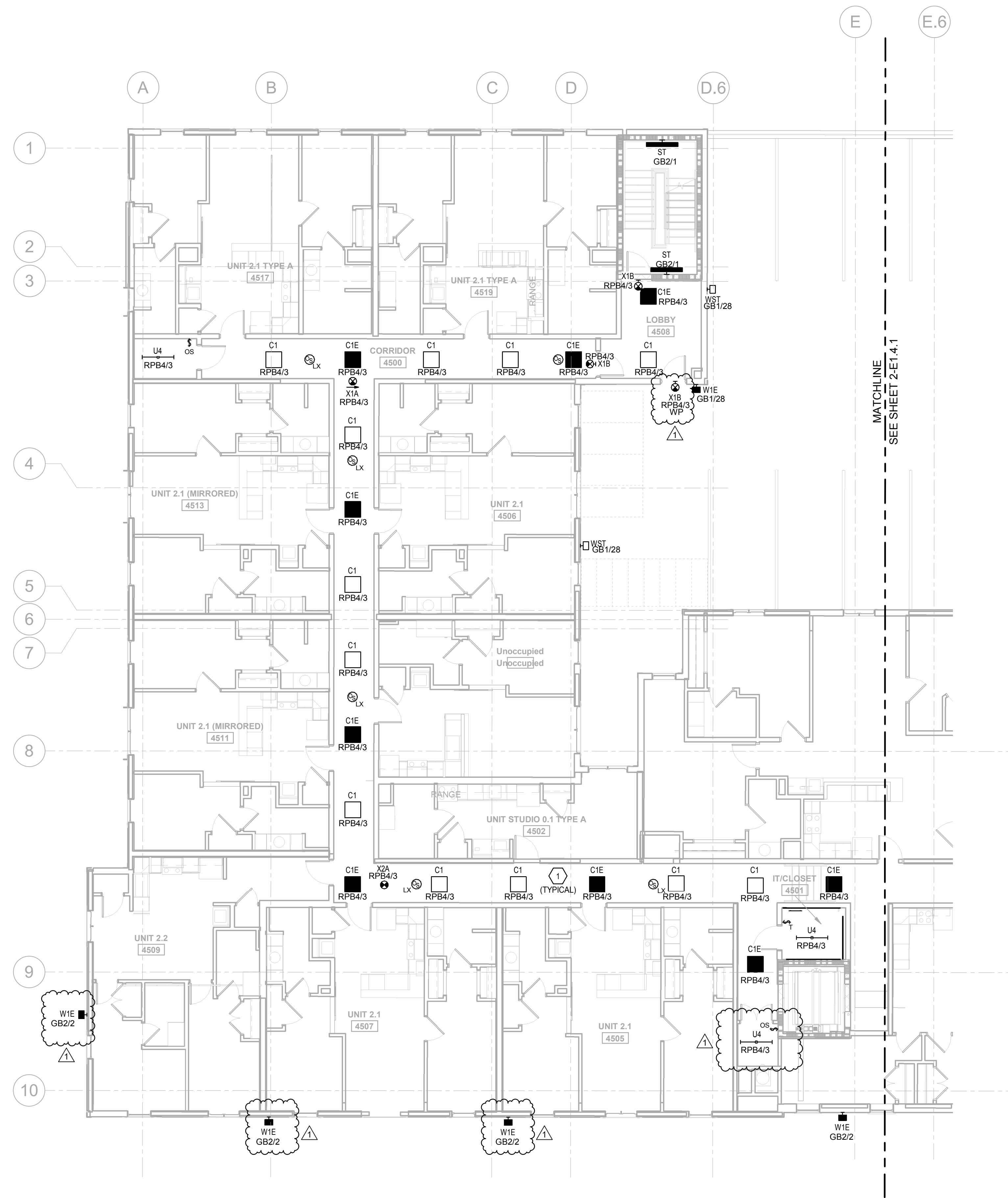
LIGHTING PLAN - BLDG 5 - FLOOR 4 SCALE: 1/8" = 1'-0"
